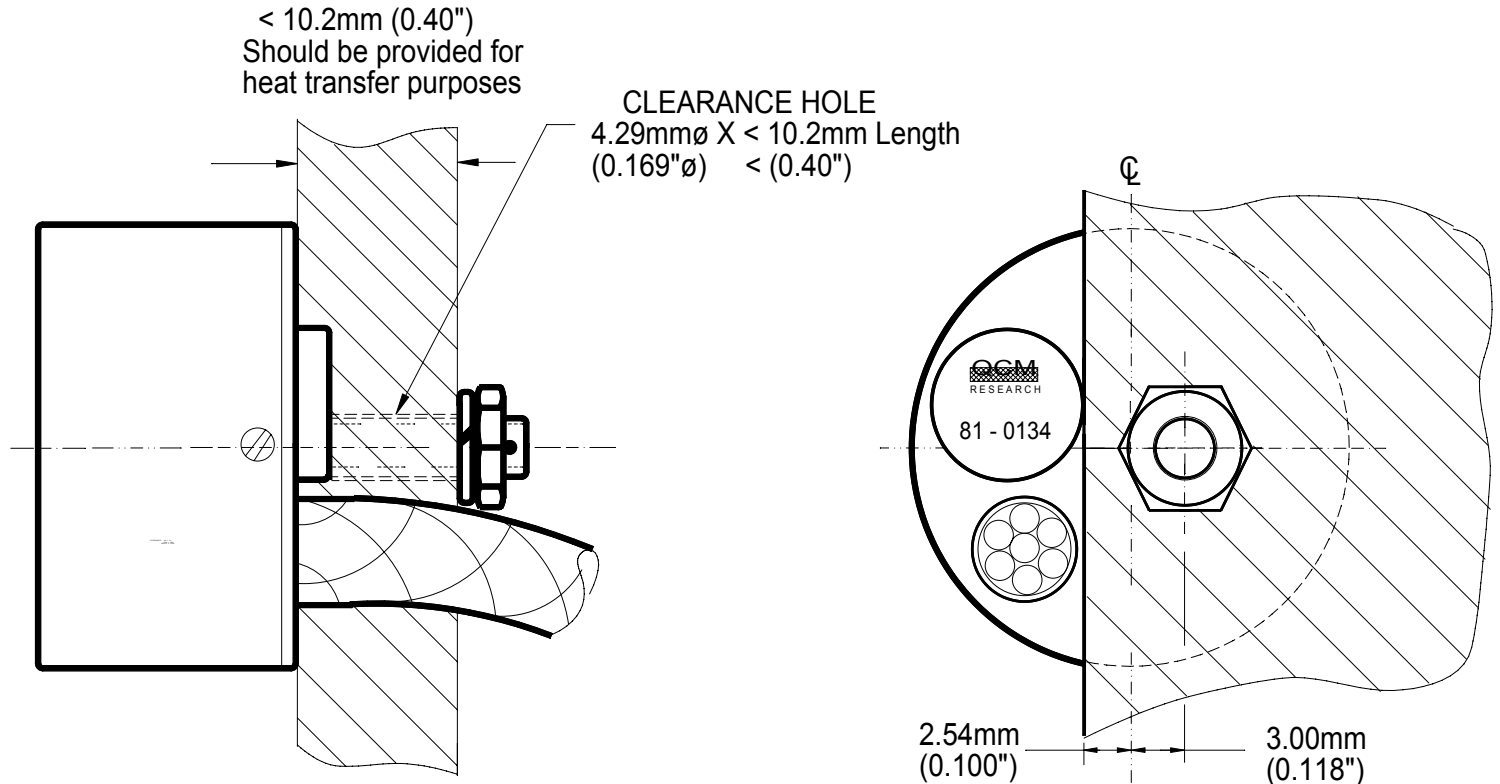
Heat Sink Partial Coverage
