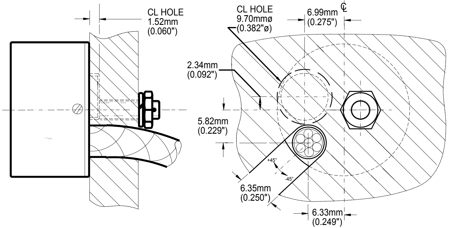
Heat Sink Entire Area Coverage
