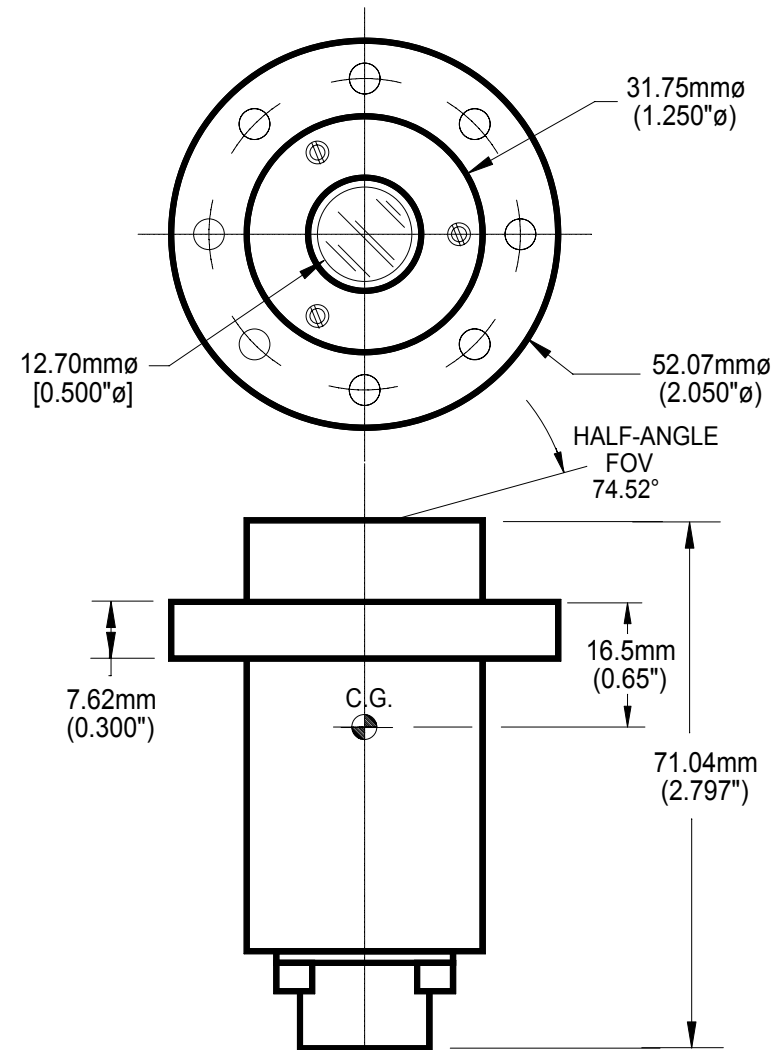
MK 10 TQCM Sensor (WT: 120 grams)
